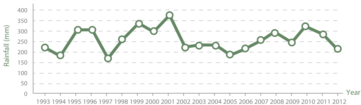
Figure 3. Makassar Rainfall Intensity.
