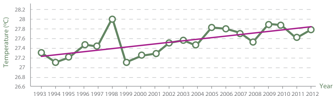
Figure 4. Makassar Average Temperature 1993 - 2012.
